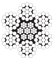
6 x 19 S
